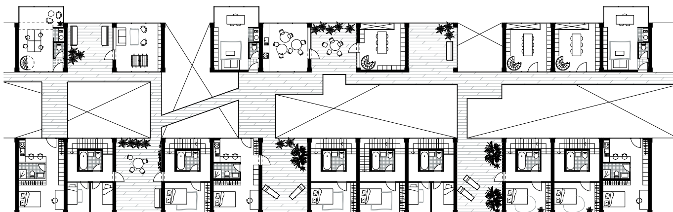
3rd floor 1/100
