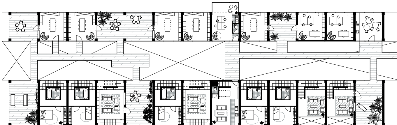
2nd floor 1/100
